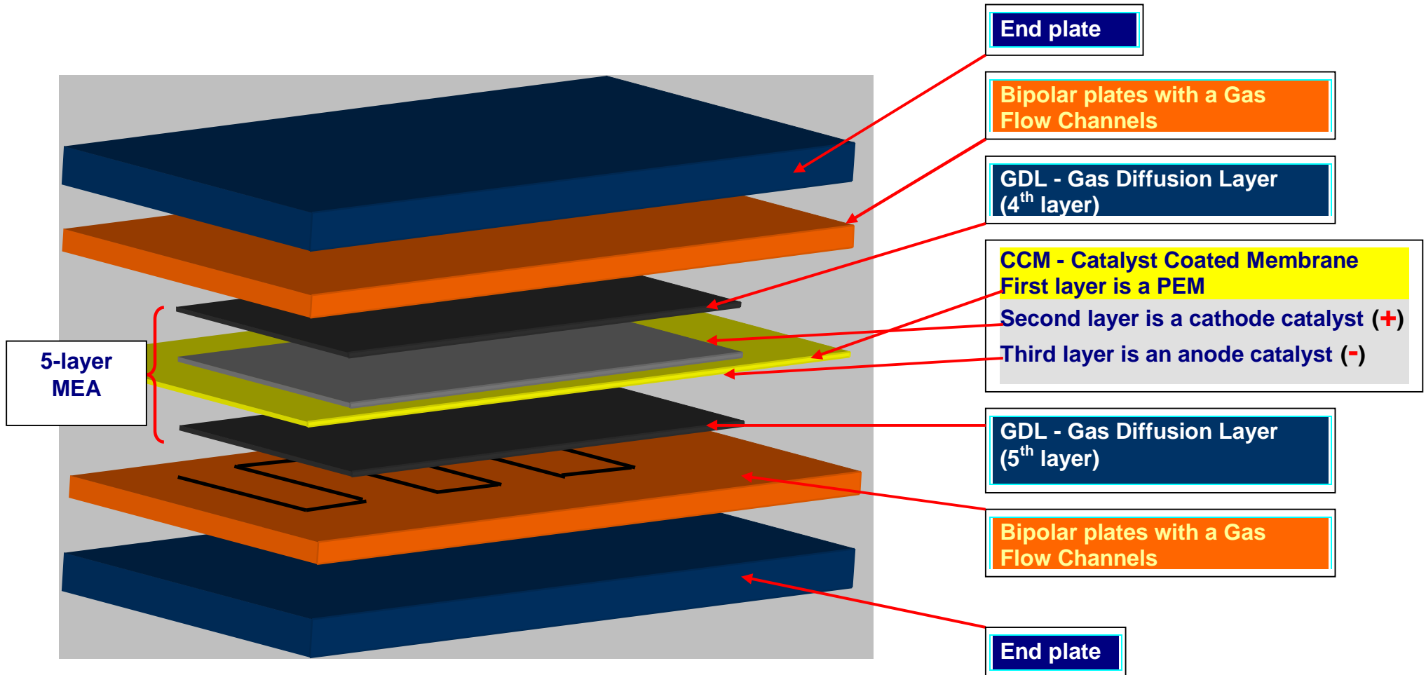
Fig.1 Exploded view of benchmark's PEM Fuel Cell (with 5-layer MEA)
